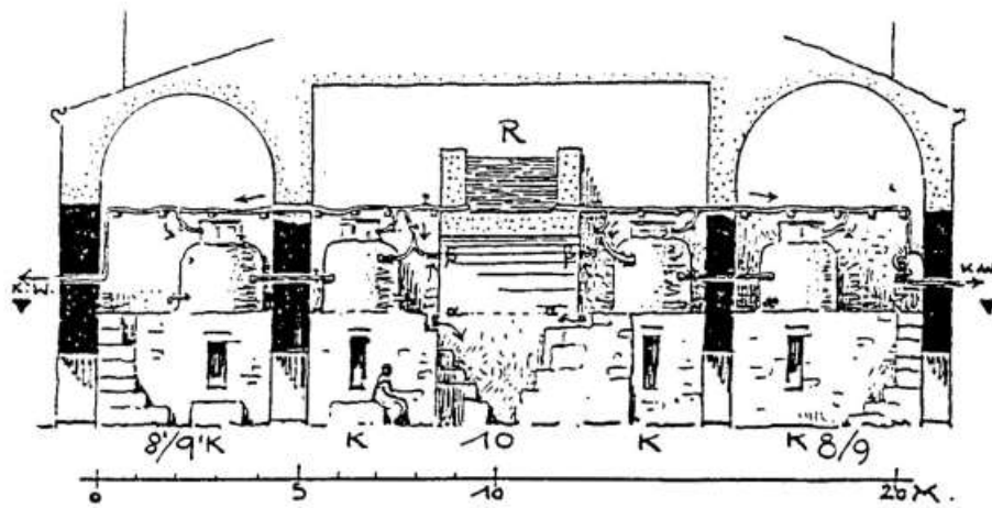
27. Lambesis : boiler room in baths, showing four boilers (Krenchker)
