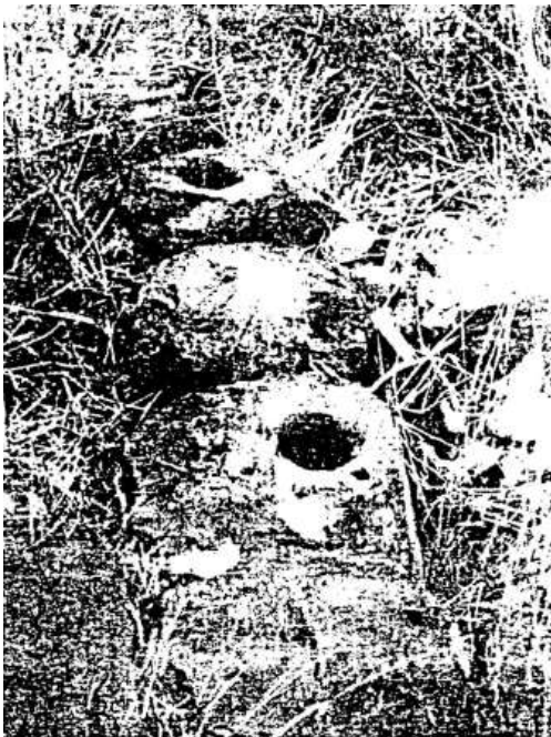
11. Hippos (Susita), Israel: stone sipone pipe in situ. The stone block have been left only roughly dressed, but again regularly carry holes on top, giving access to the pressure channel within (for air venting? Maintenance?) (see Fig. 12)
