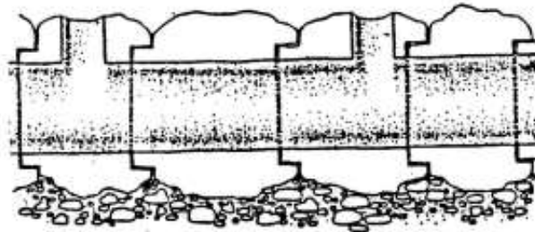
12. Hippos (Susita), Israel: stone siphon piping, in plan, elevation and section, showing (vent?) holes (Y, Peleg)
