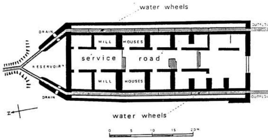
20. Barbegal : reconstructed plan, partly conjectural.
