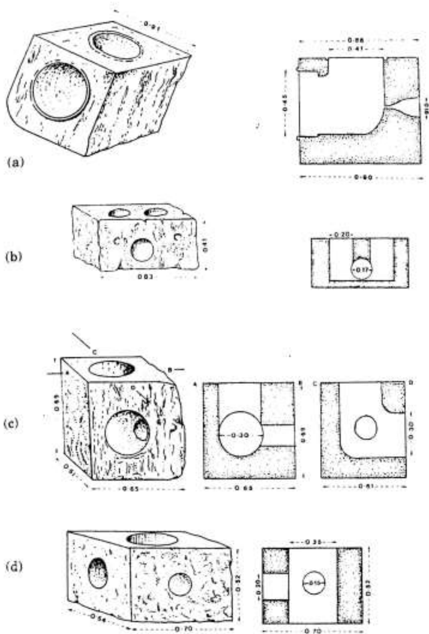
8. (a) Laodicea angle block from stone pipeline showing (section), possible air vent hole; (b), (c), (d) Smyrna : various angle and junction block from stone siphon piping (Weber)
