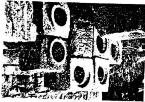
6. Ephesos: blocks from a stone pressure pipe, piled in the agora; some (e.g. top centre) carry in the side a vent(?) hole.
