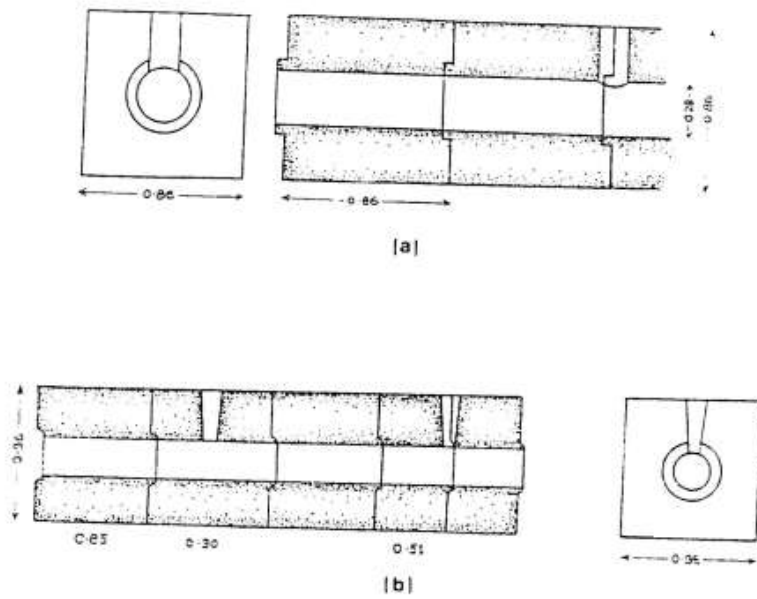
10. Stone pipeline blocks showing (vent?) holes, from (a) Aspendos; (b) Laodicea (Lanckoronski, Weber)
