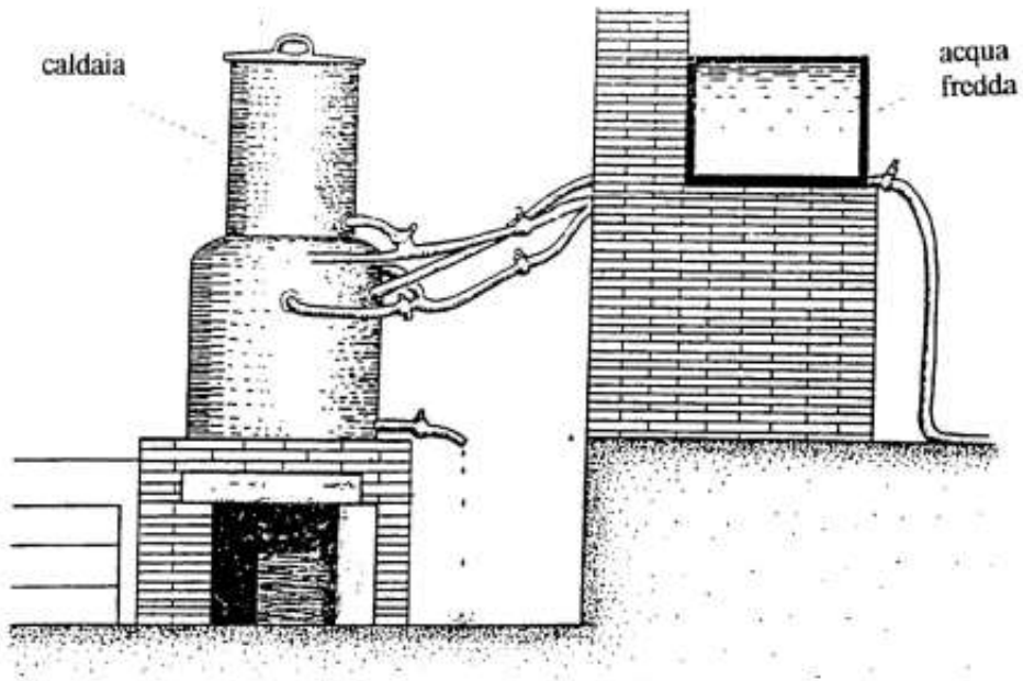
28. Boscoreale (near Pompei): above: heating boiler jør domestic baths: below: close-up of piping: 7= cold water supply; 2 = boiler; 8 = warm water delivery pipe (Kretzschemer).
